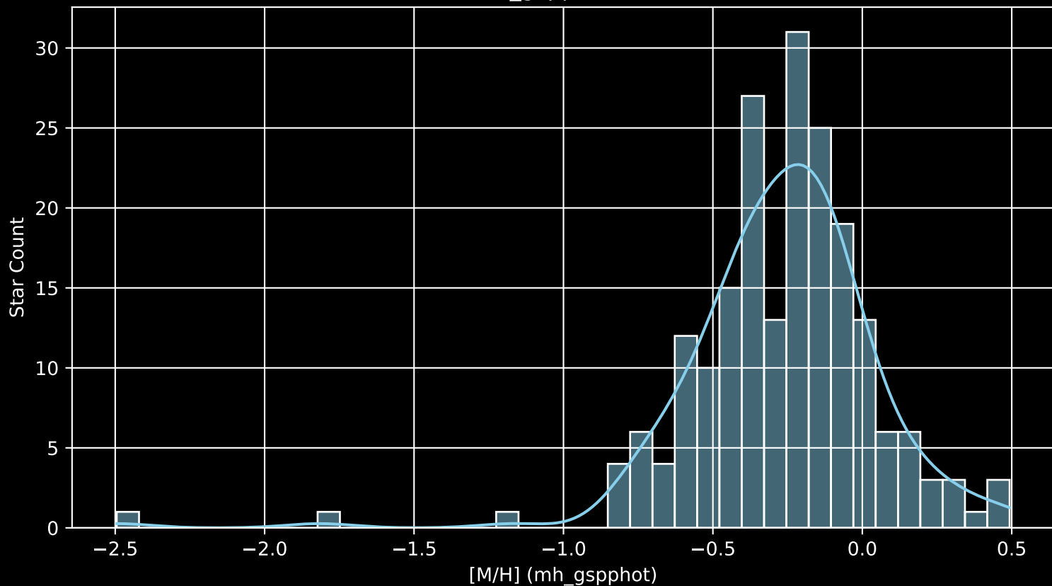
APOGEE DR17 Field: [K2_C3_049-49 [M/H] (mh_gspphot) (n= 204)
