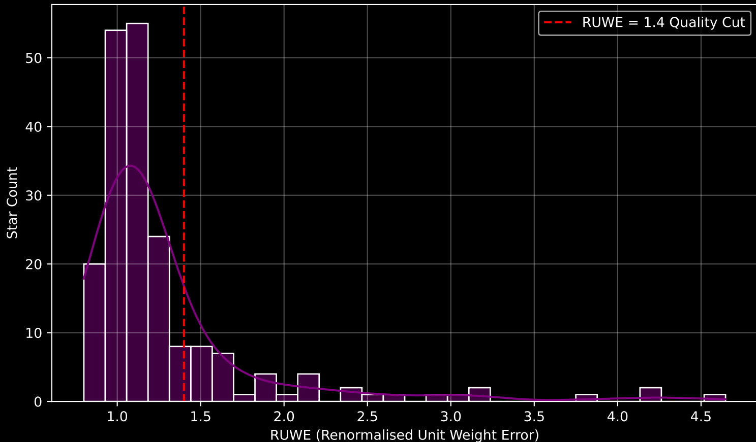
GAPOGEE DR17 Field [K2_C3_049-49] RUWE Distribution (n= 198)
