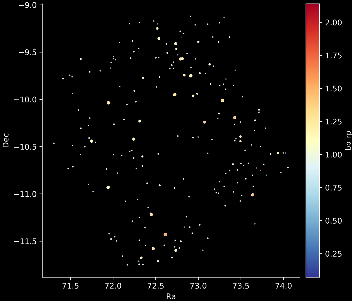
APOGEE DR17 Field: [K2_C3_049-49] Stars: 205
