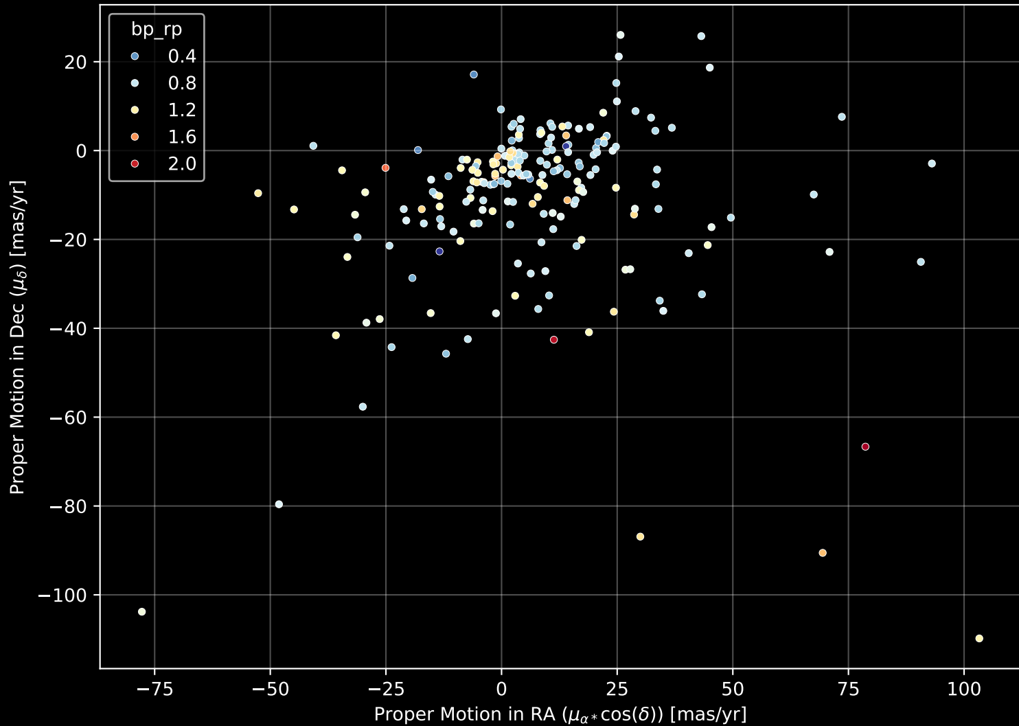
APOGEE DR17 Field: [K2_C3_049-49] Proper Motion Diagram (n= 205)
