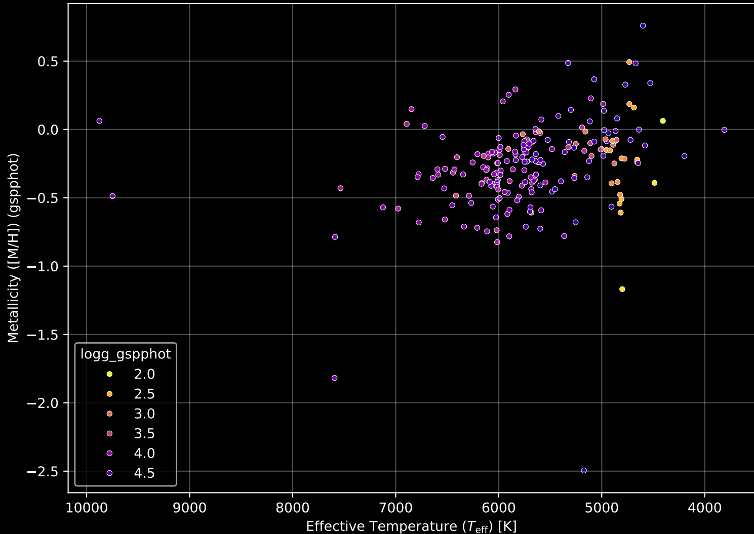
APOGEE DR17 Field: [K2_C3_049-49] Stellar Population Parameters (n= 205)
