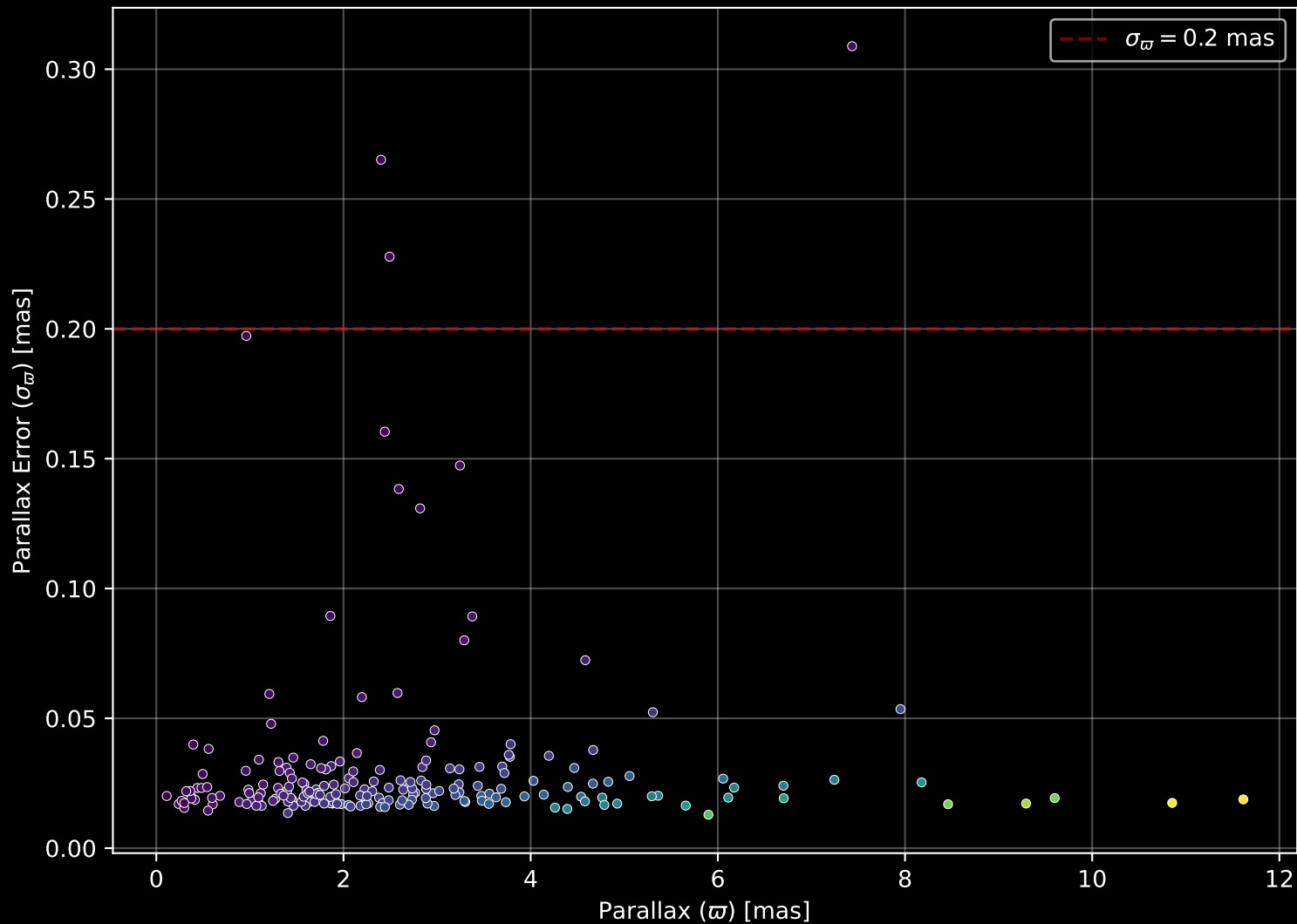
APOGEE DR17 Field: [K2_C3_049-49] Parallax Quality (n= 205)
