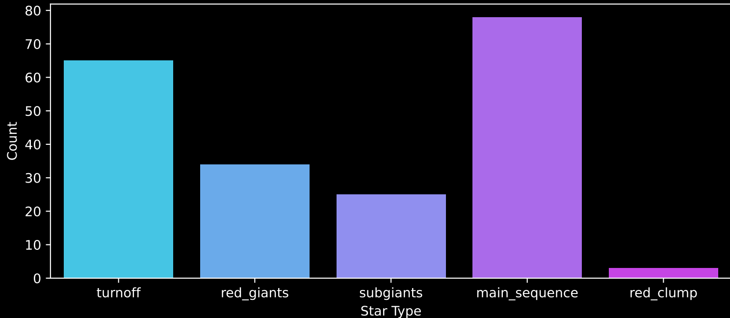
APOGEE DR17 Field: [K2_C3_049-49] Count plot of Star Type
